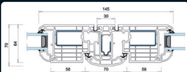
French Door Mullion
