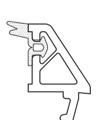
096-04 Bead 28mm Glazing
