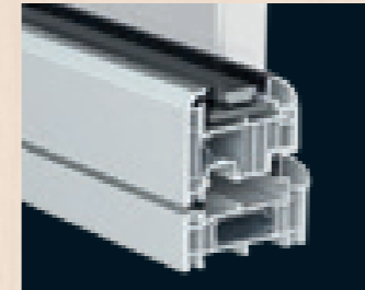
6 chambered sash for high thermal efficiency
