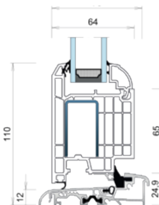
Low Threshold
