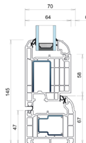
Std Threshold
